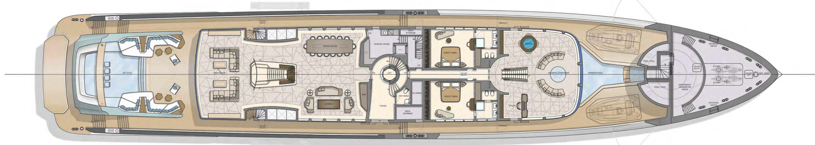
MAIN DECK
